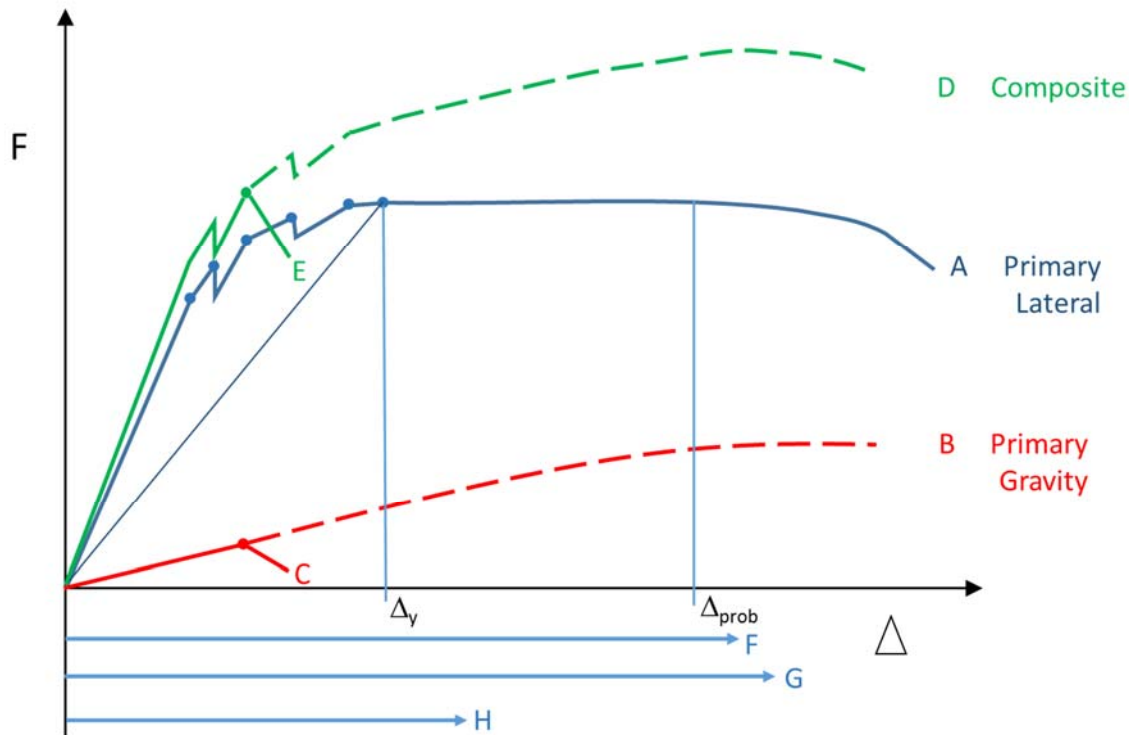
Figure A3.2: Force-deflection relationships for systems and individual elements
