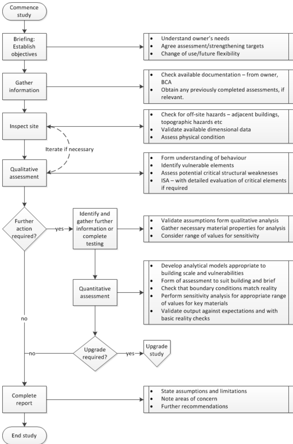
Figure A4.1: Generalised Assessment Process Flow
