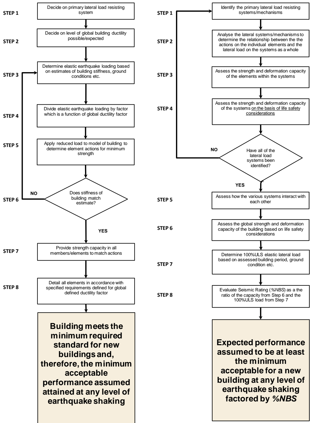
(a) Traditional Design Approach
