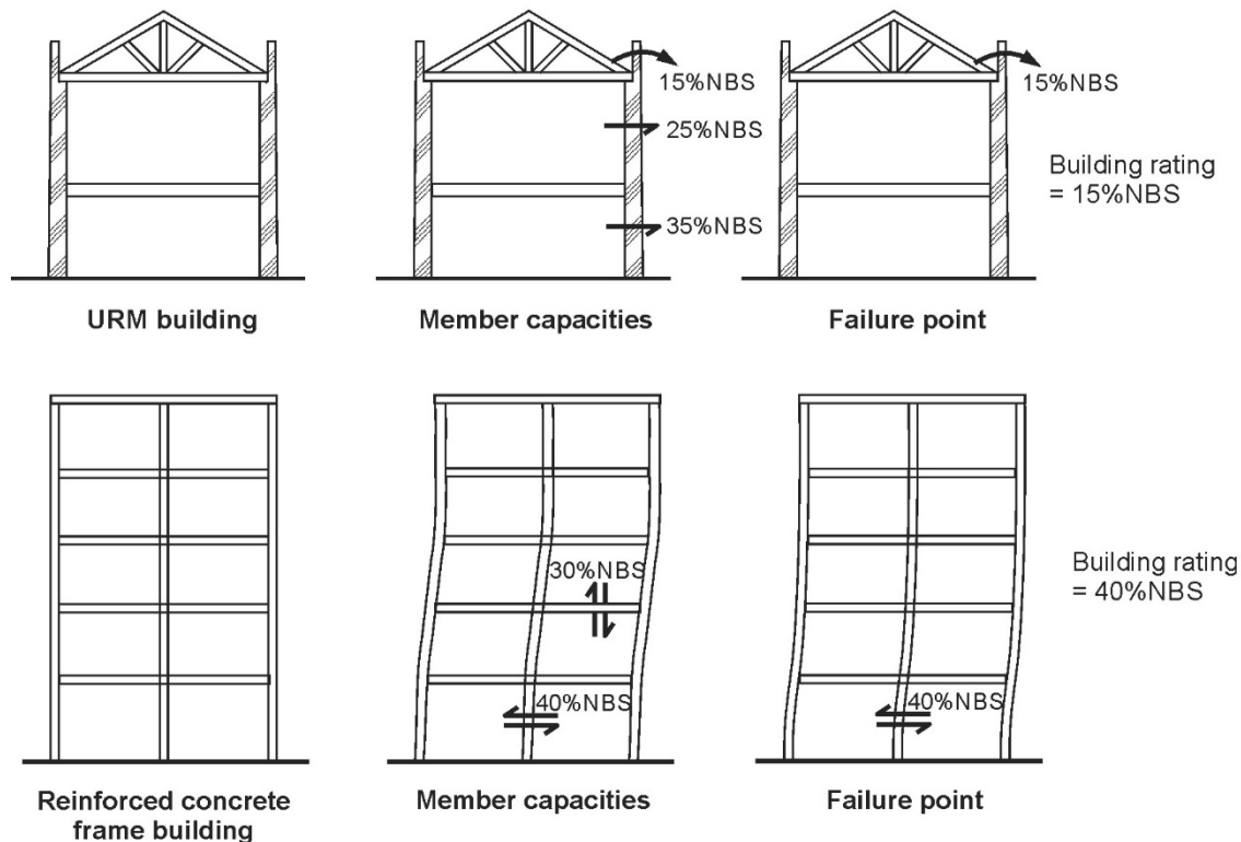
Figure A3.3: Illustration of the Calculation of %NBS for the Building as a Whole
