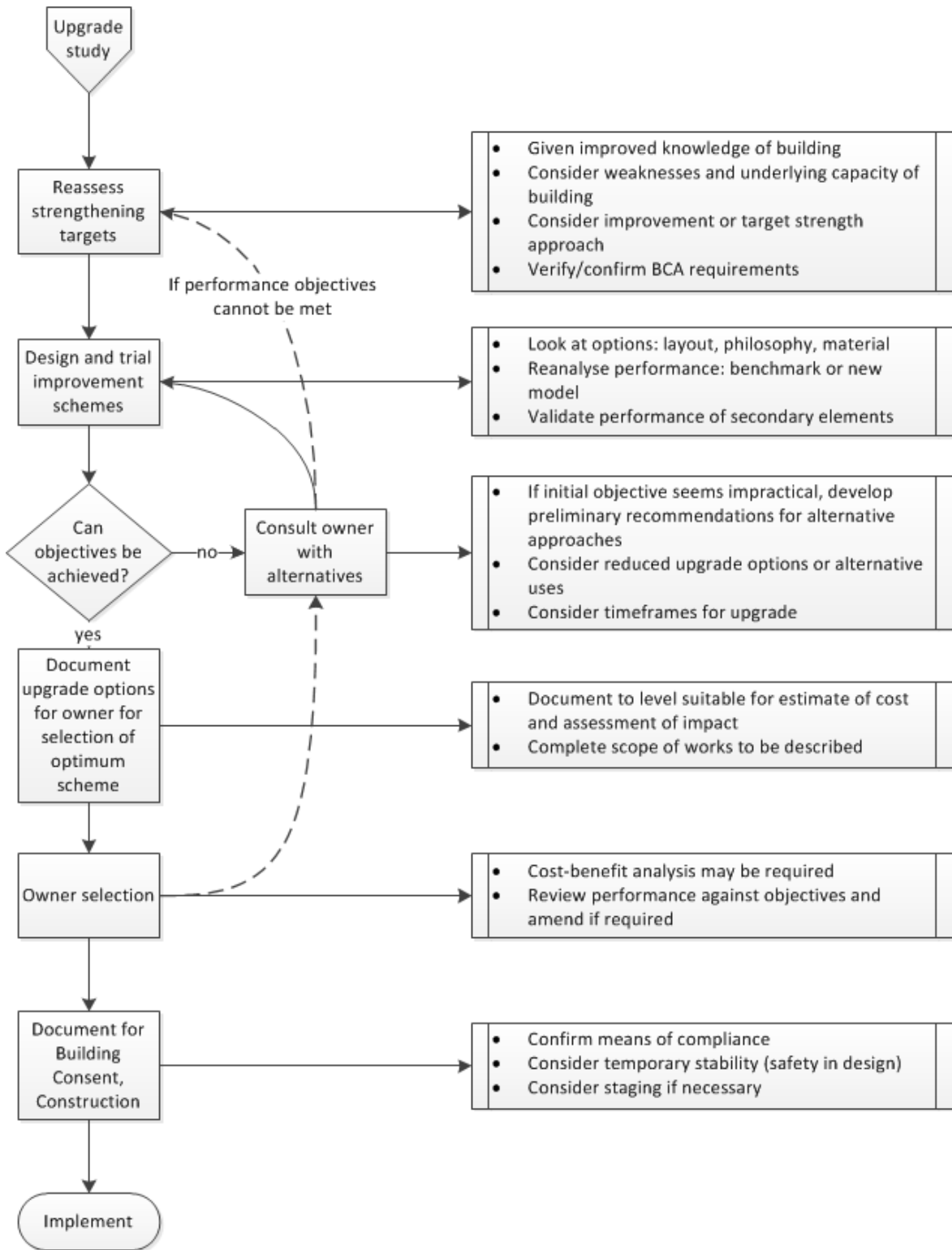
Figure A6.1: Generalised Seismic Upgrade Process Flow
